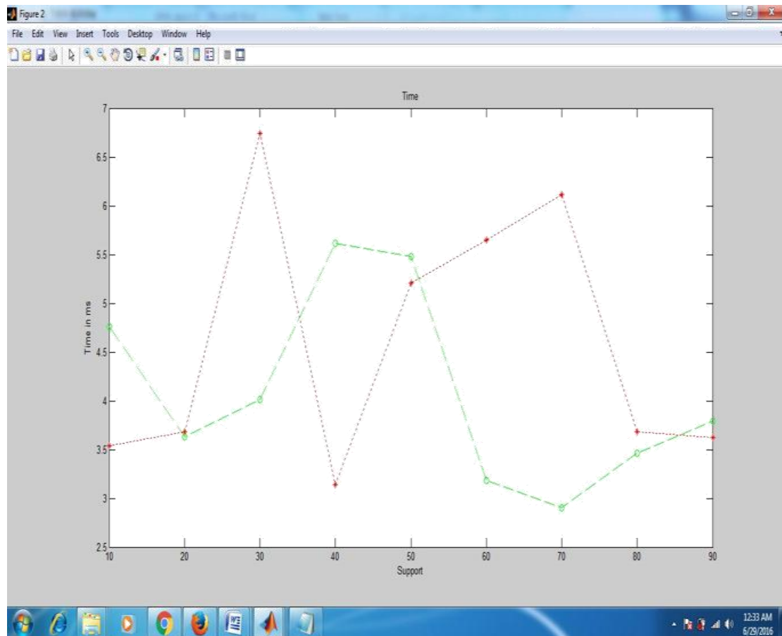
Figure 4: Comparative time complexity of HMCC and GA-MCC
