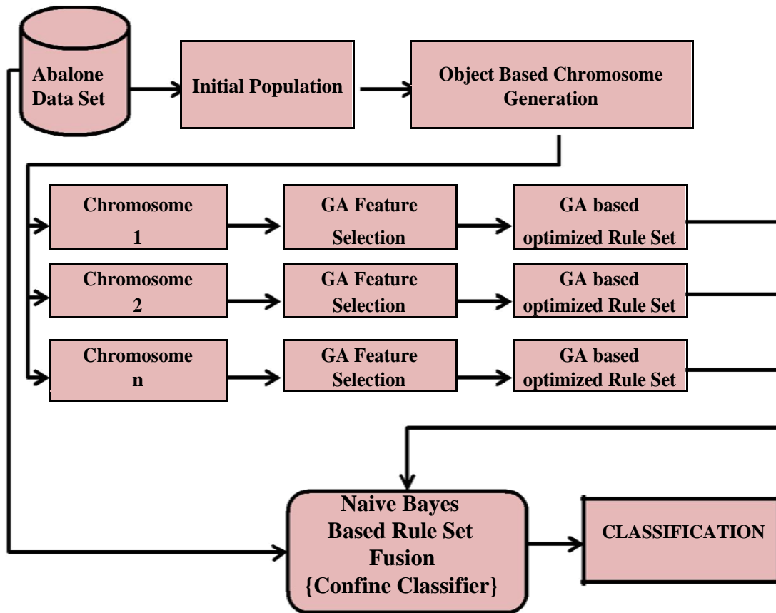
Figure 2: Proposed Model For GA-MCC
